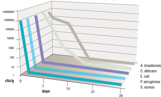
O/W-emulsion with organic acids + dermosoft® surface active material (0,3%) at pH 5,3
